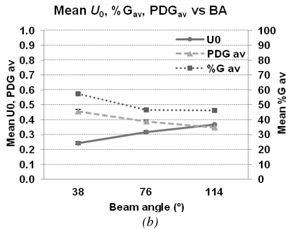
(b) Figure 8 Graphs showing the relationship between the arithmetic mean of the output variables and the most influential input variables, i.e. (a) the space availability and (b) the beam angle. The error bars indicate 95% confidence level.
