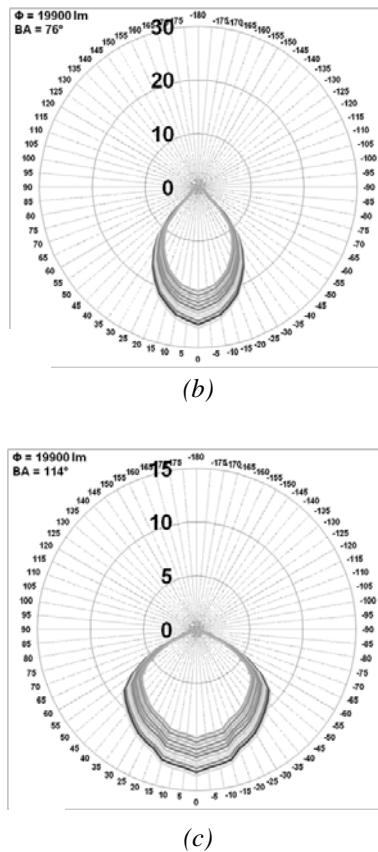
Figure 4 Examples of polar diagram of luminous intensity (in candela) of the light sources resembling the sky, with beam angle of (a) 38°, (b) 76°, and (c) 114°
